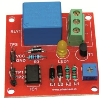
WATER LEVEL CONTROLLER
