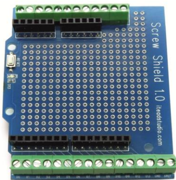
SCREW SHIELD FOR UNO & MEGA
