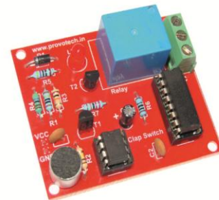
CLAP SWITCH
