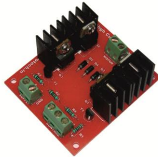
HIGH CURRENT STEPPER MOTOR DRIVER
