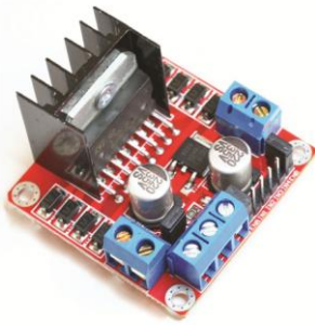
L298N MOTOR DRIVER BOARD
